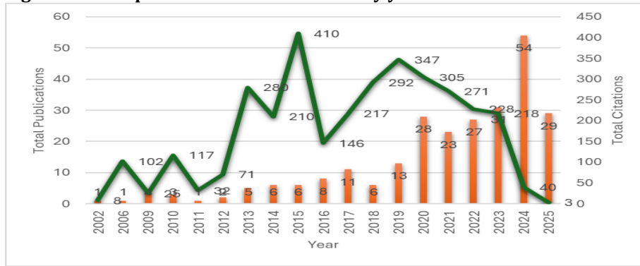
Figure 2: Total publications and citations by year
