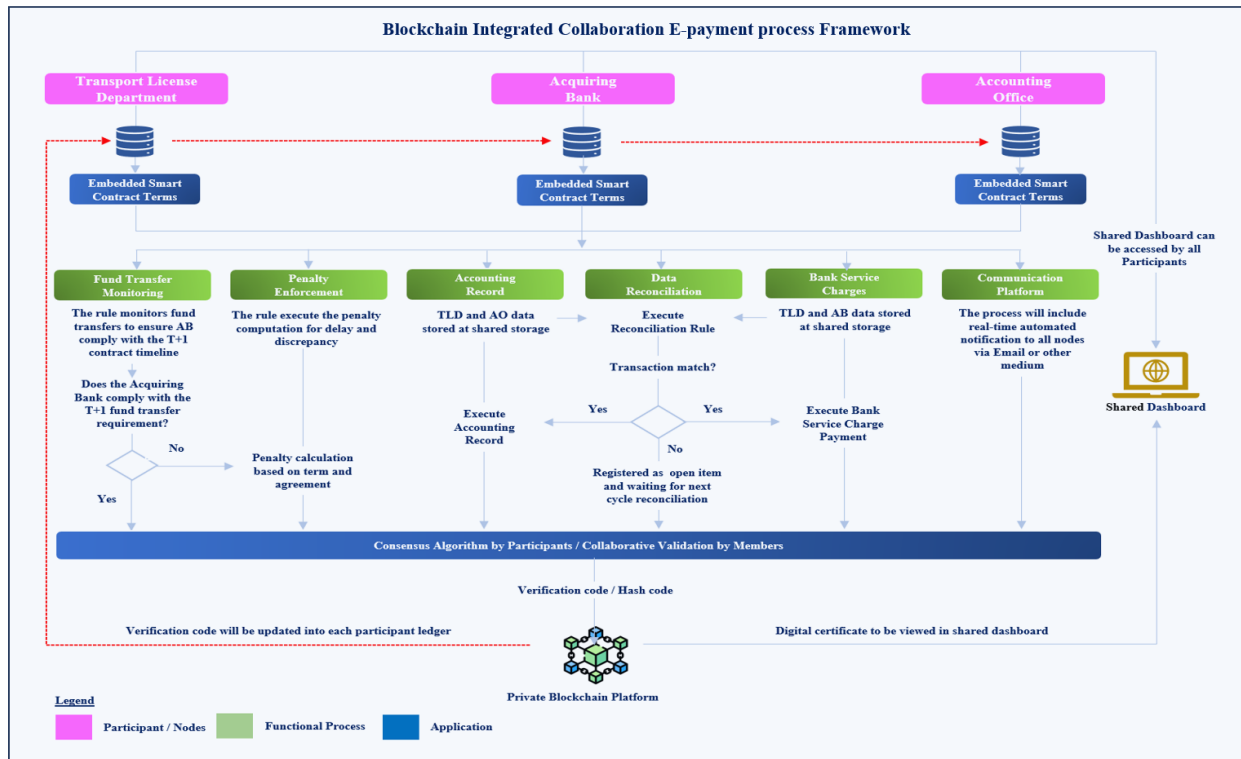
Figure 2: Blockchain-Enabled Collaborative E-Payment Framework (BICEF)
