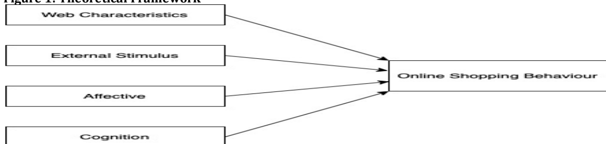
Figure 1: Theoretical Framework
