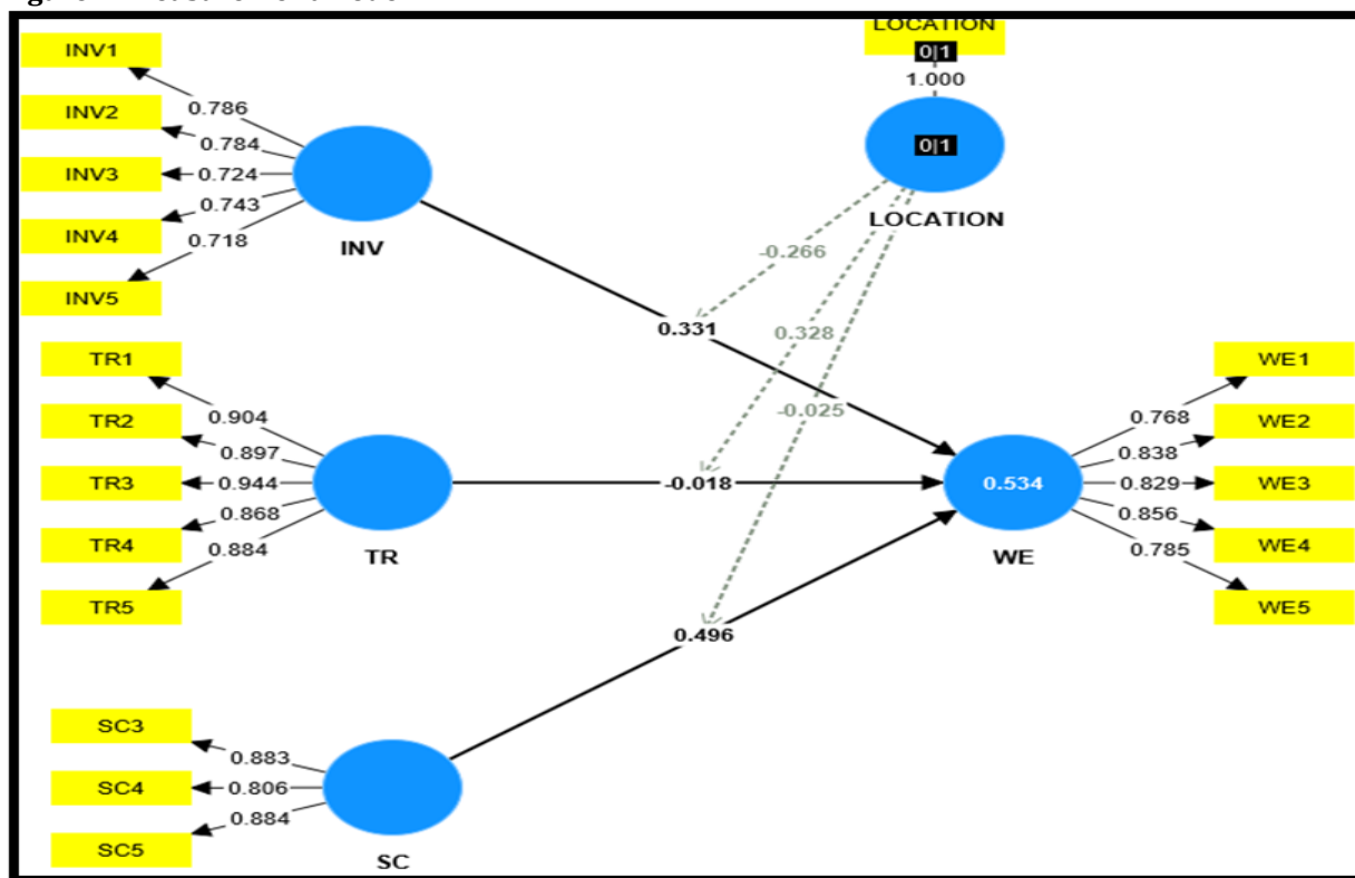
Figure 1: Measurement Model
